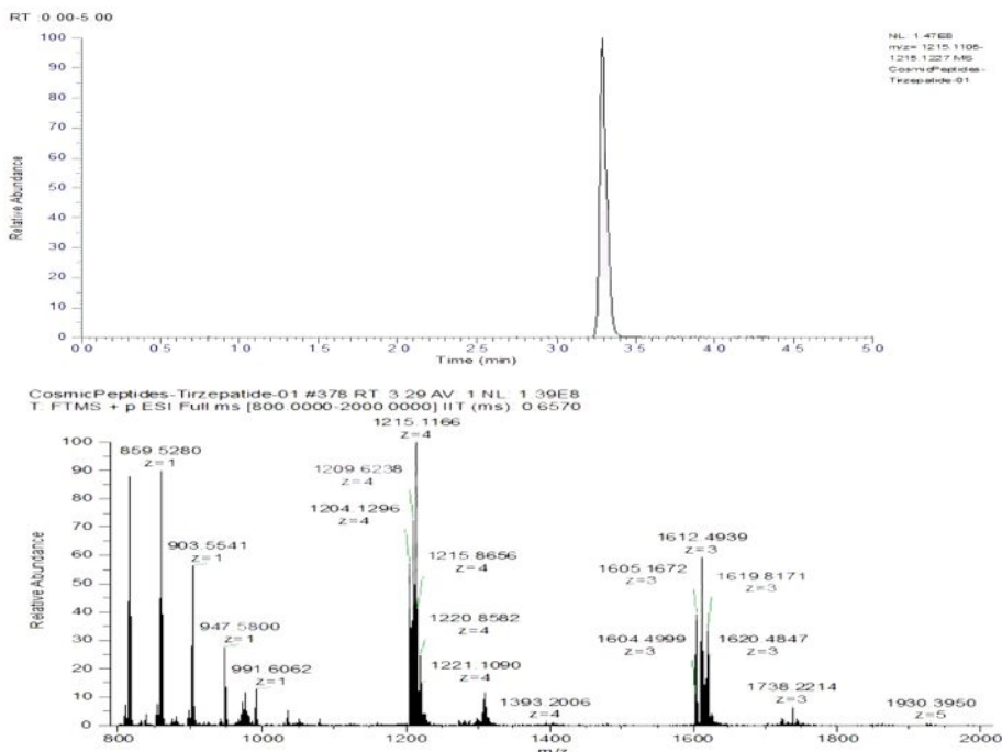
LC-MS Chromatogram: Retention Time and Peak Analysis
